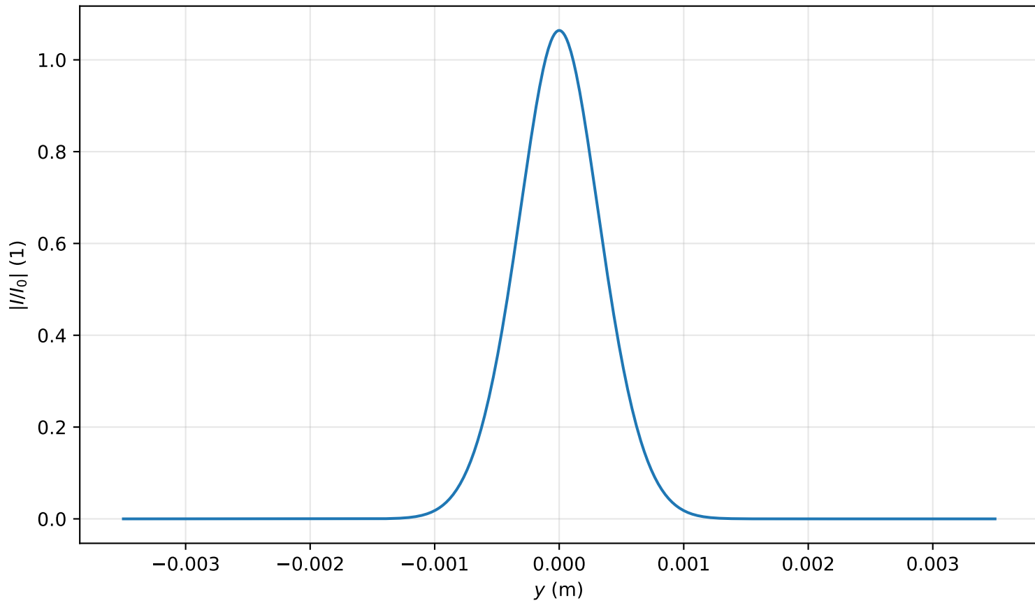
Intensity profile I(x=0, y, z=0.318)/I_0 , P_{in}=0.9P_{cr} , artificial time
